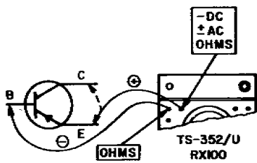
A. FORWARD EMITTER DIODE TEST
