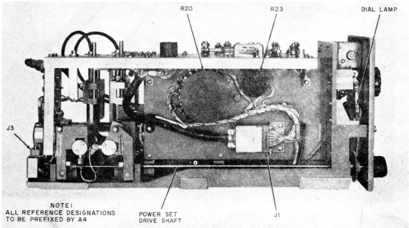
Figure 3-7. RF Oscillator Section, left side view.
