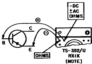
C. REVERSE EMITTER DIODE TEST
