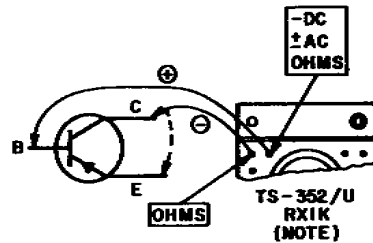
B. FORWARD COLLECTOR DIODE TEST
