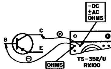
D. REVERSE COLLECTOR DIODE TEST
